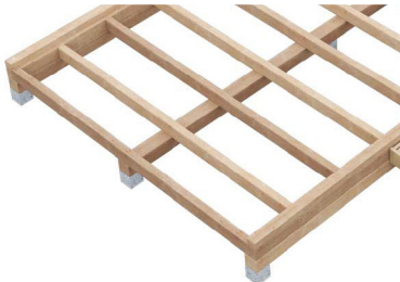
Floor framing 100x50 H3.2, 100x100 H4 bearers
